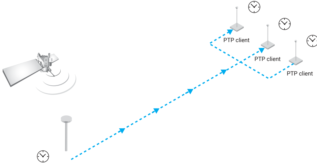
Figure 1. Network synchronization relying on 1588 PTP and SyncE
