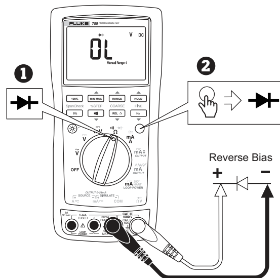
Good Diode
