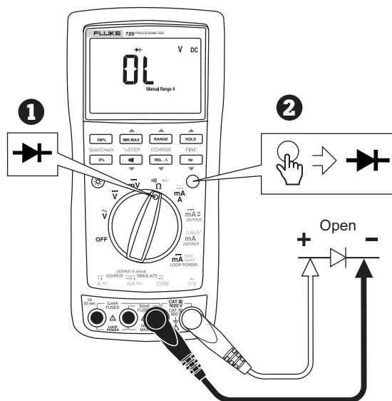
Bad Diode
