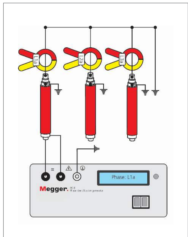
Basic circuit diagramm of a phase identification
