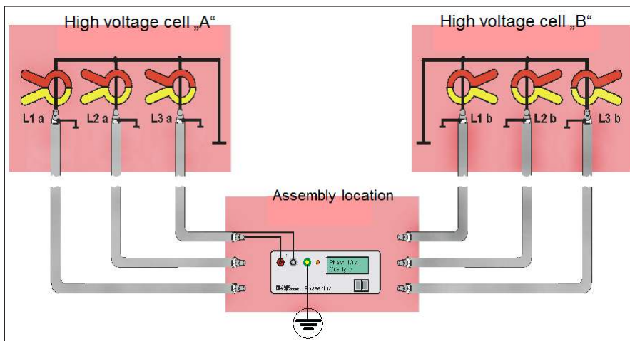
Connection with optional transceiver clamps coded (L1b, L2b, L3b)
