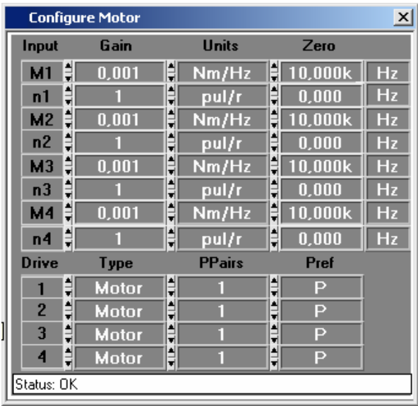
Figure 4-5. Configure Motor
