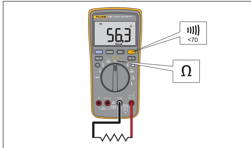
Figure 3. Measure Resistance/Continuity
