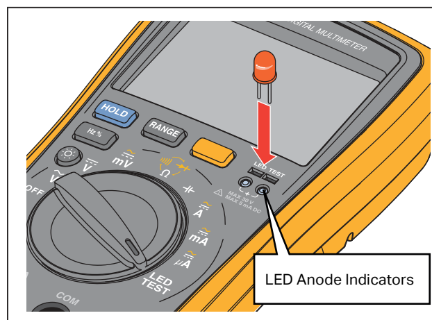
Figure 4. LED Test Sockets
