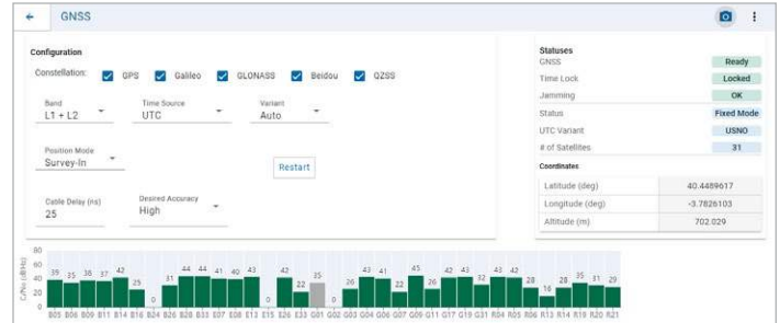
Figure 9. GNSS supported satellites.
