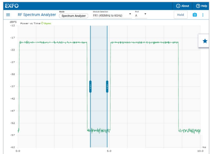
Figure 7. TDD gated sweep.
