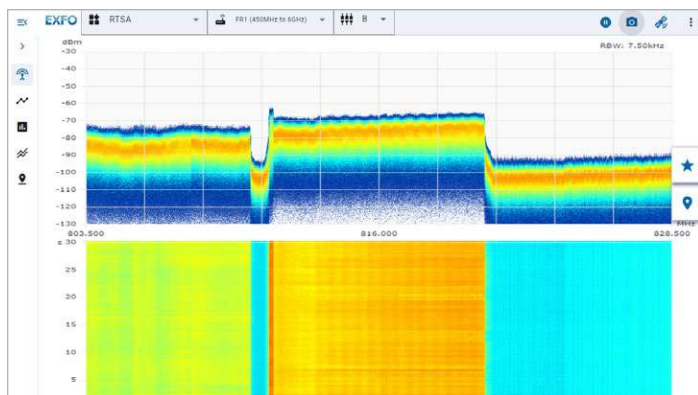
Figure 2. Real-time persistence spectrum with waterfall diagram.
