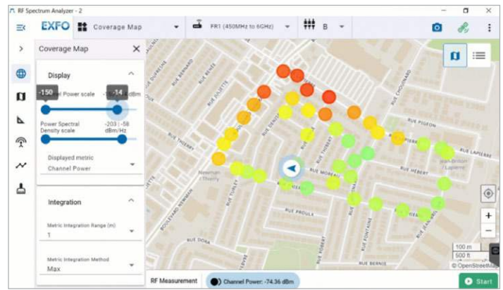
Figure 13. Coverage mapping for channel power.
